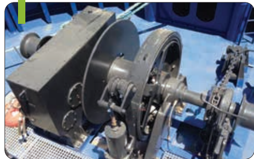
Combined Fore Towing Winch
