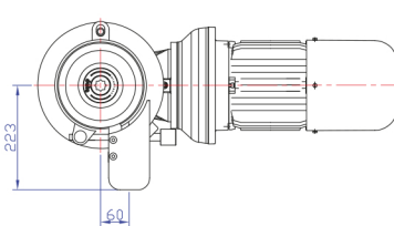
Electric motor drive 90° (380 V)
