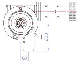
Electric motor drive 90° (24 V)
