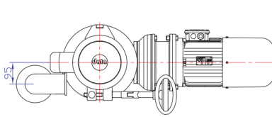
Electric motor drive 90° (380 V)
