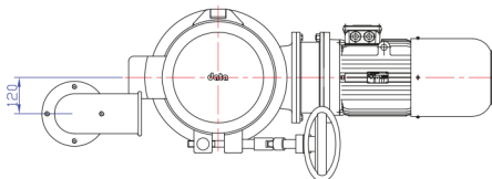
Electric motor drive 90° (380 V)
