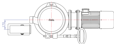
Electric motor drive 90° (380 V)
